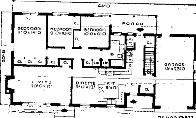
A SMALL HOUSE PLANNING BUREAU DESIGN NO. C-522
